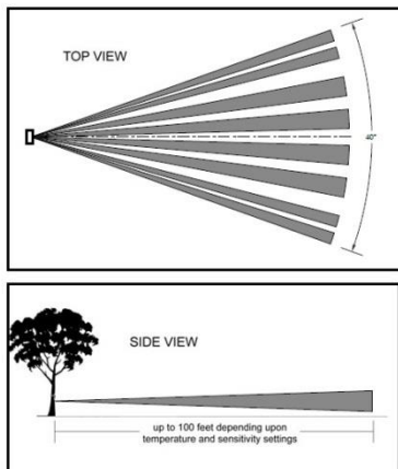
PIR MOTION DETECTOR COVERAGE AREA
