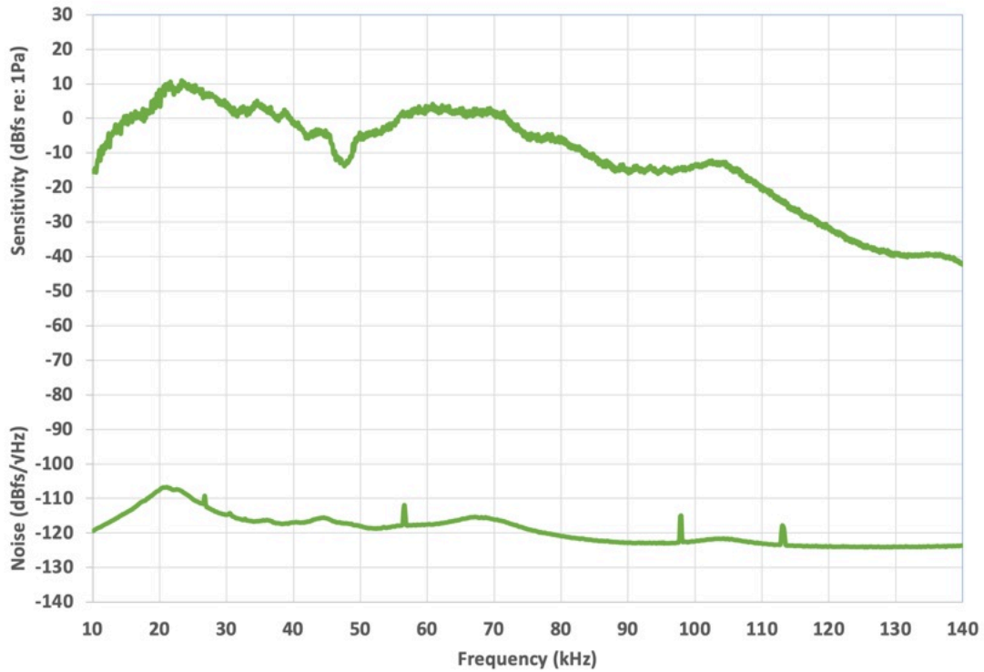
Figure 15. Sensitivity and Noise of the SMART System with SMART MIC-1
